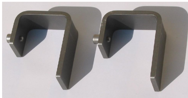
photo 4: HOOKS FOR FLYING INSTALLATION (OPTION)
